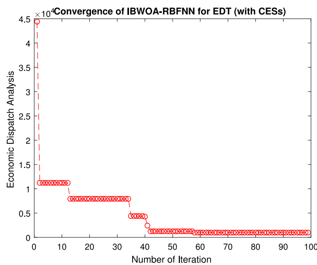
Fig. 12. IBWOA-RBFNN convergence for Case Study-I (including CESs).
